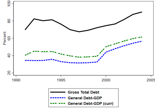
Figure 15: Comparison of BP-DG
