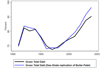
Figure 16: Comparison of BP-DG (replication)
